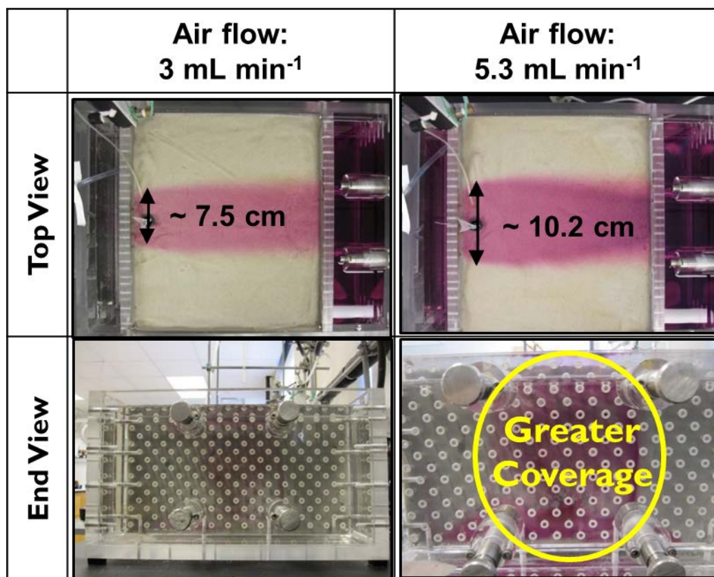
Figure 40. Influence of air rate on the lateral spreading
