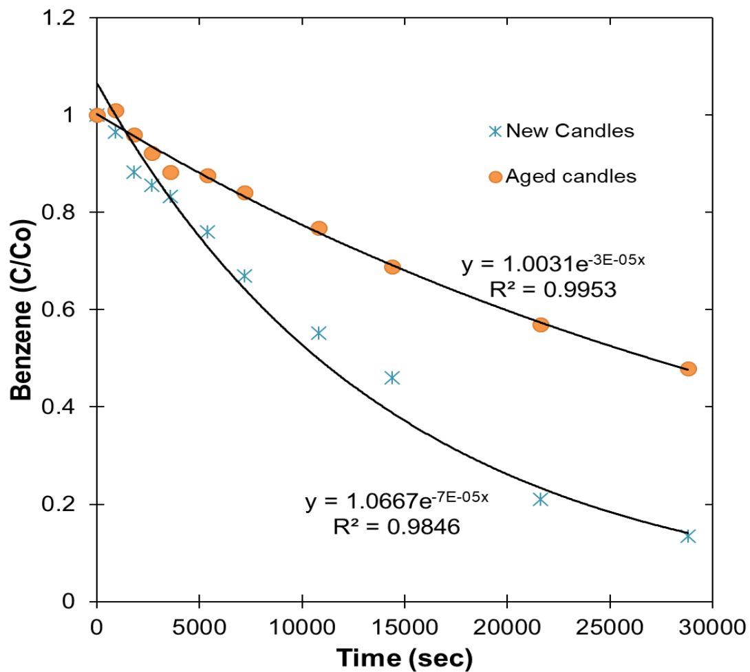
Figure 37. Benzene concentrations ( C_0 = 0.5 \text{ mM} ) over time with new and 48-hr aged persulfate and zero-valent iron candles
