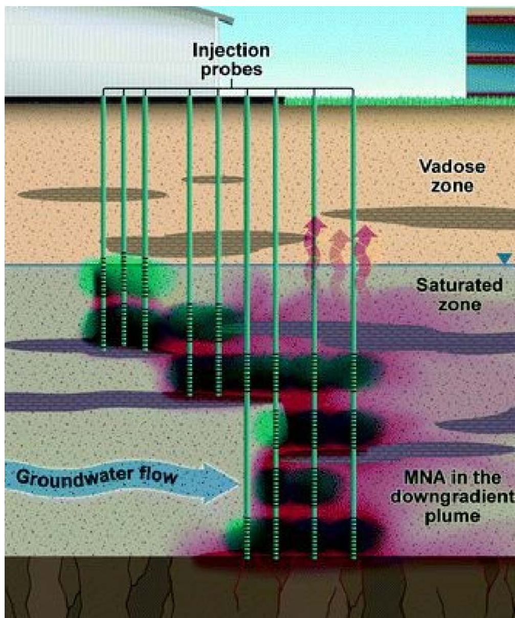
Figure 2. Illustration of ISCO to treat contaminated groundwater
