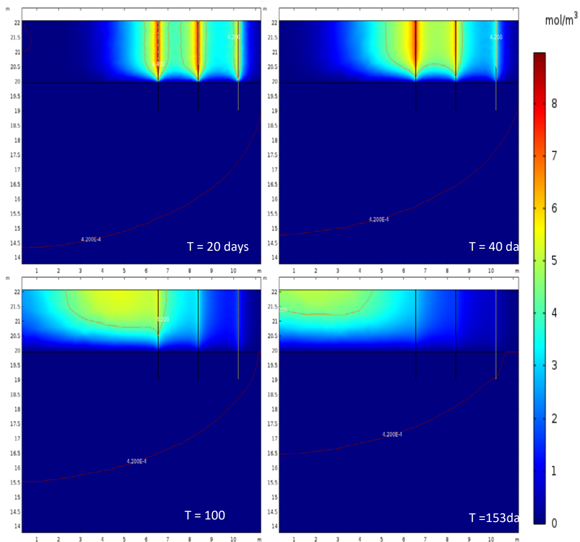
Figure 34. Simulated concentration of sodium persulfate from first column of candles at 20, 40, 100, 153 days in the two-layer model (flow direction is from the right to left)
