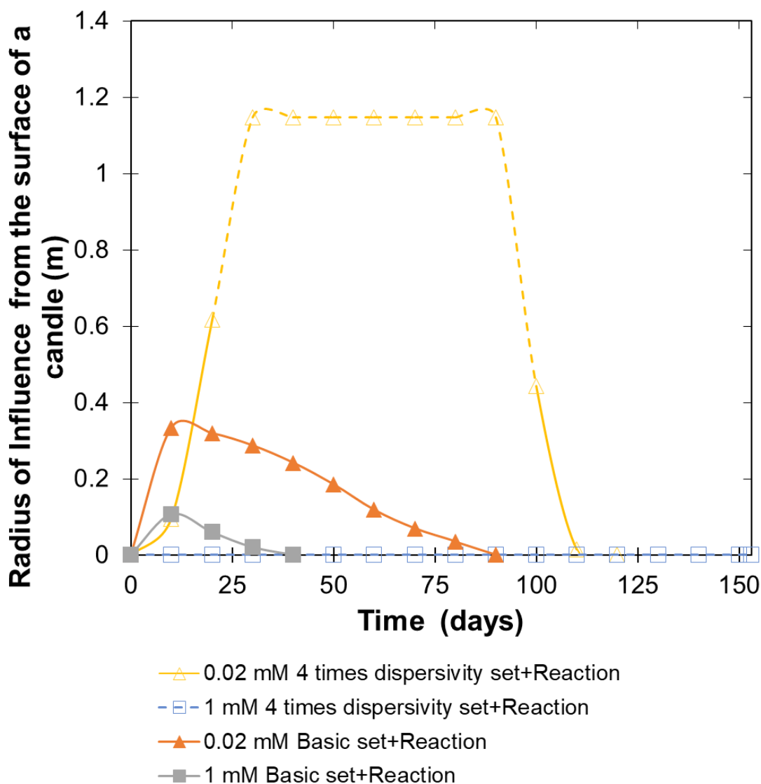
Figure 54. Aeration & Basic set: The radius of influence of a candle on the right of the first row in the transverse direction over time via various concentration of benzene. Dash lines meant the connection had artificial data point where the radius of influence was zero or its maximum was out of the simulation domain.
